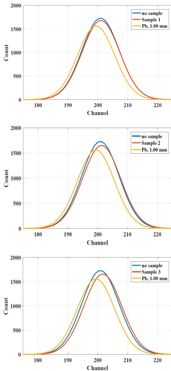
Fig 2. Smoothened graphs for the photon counting and the calculation of the samples' ability for \gamma - ray attenuation; pure PVC/0 (above), PVC/20 (middle), and PVC/40 (below).
