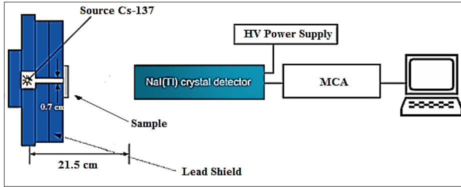
Fig. 1. Schematic view of the experimental setup.
