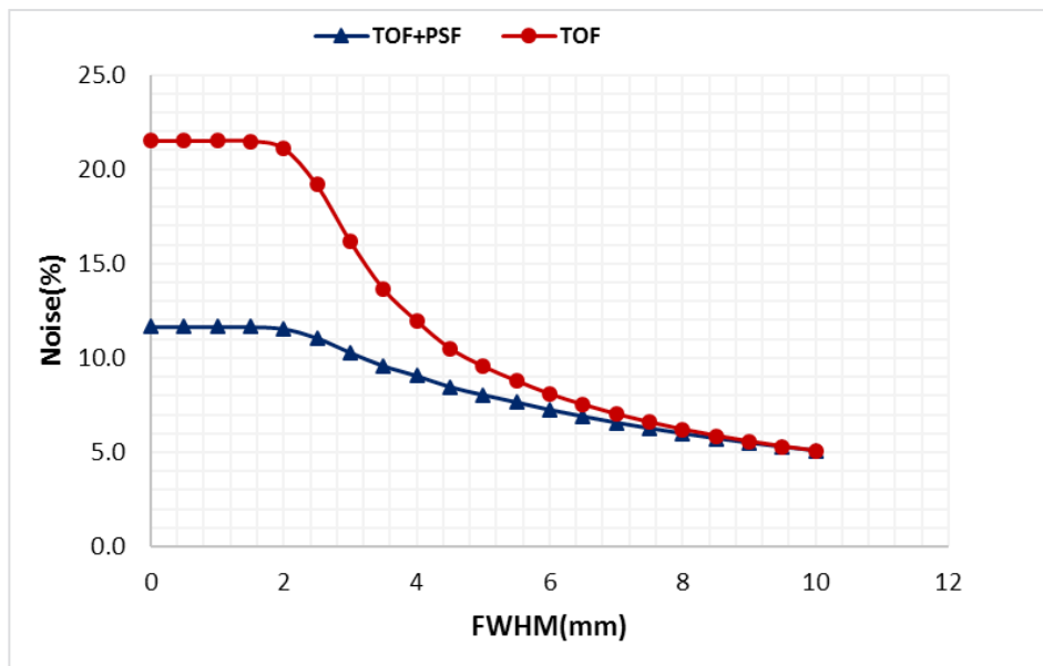
Figure 2. Noise trends against different filter size for PET images reconstructed with TOF and TOF+PSF algorithms.
