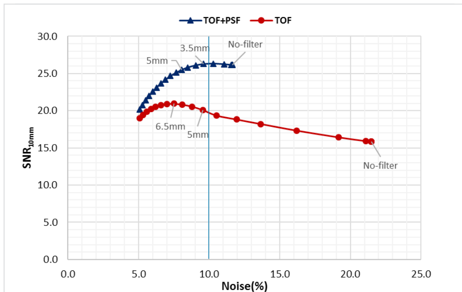
Figure 3. SNR_{10\text{ mm}} against noise for PET images reconstructed with TOF and TOF+PSF algorithms. Each point shows a filter size ranging from 0 to 10 mm with 0.5 mm increment.
